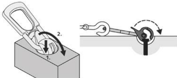
1. Engagement
